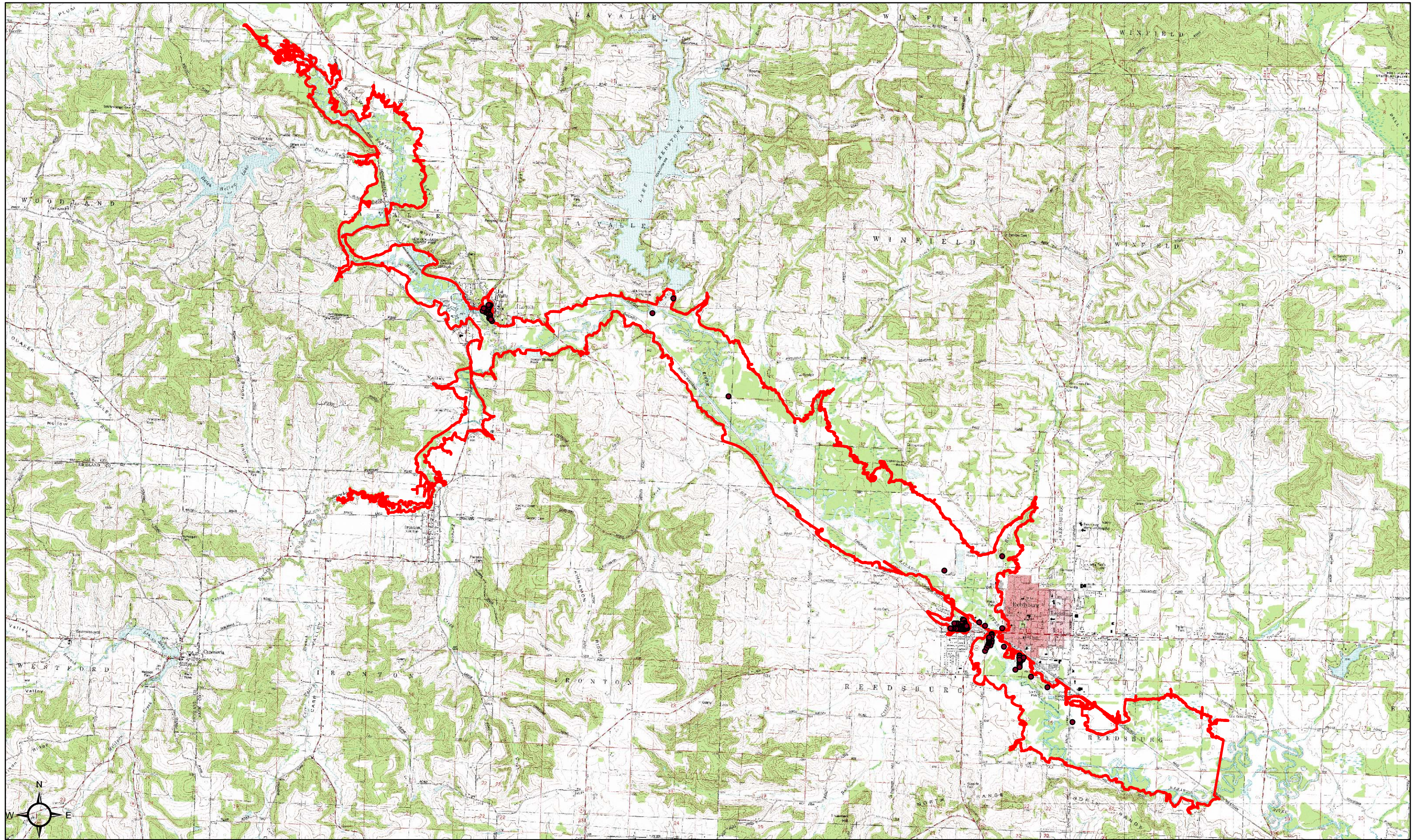
Exhibit 4 Lake Redstone Dam Hydraulic Shadow
